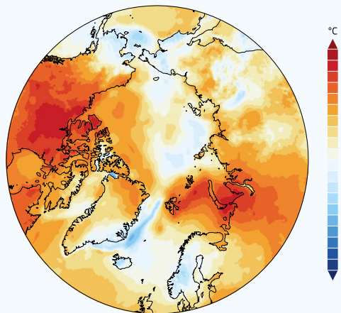
Anomalies in surface air temperature in 2023
