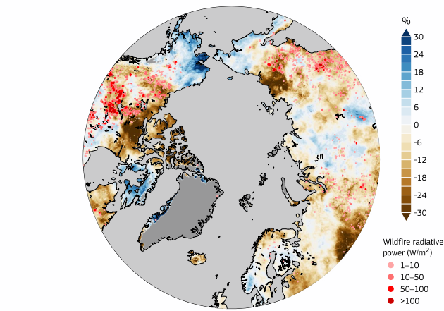
Wildfires and anomalies (%) in soil moisture in June to August 2023
