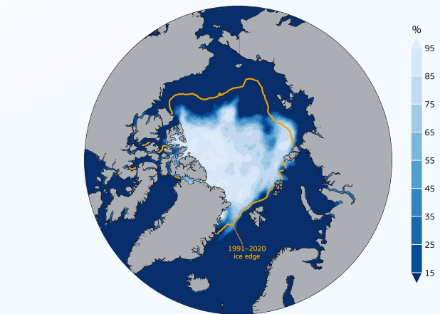
Monthly average sea ice concentration (%) in September 2023
