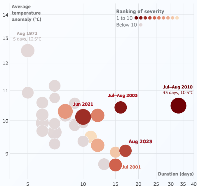
Top 30 most severe heatwaves in Europe (1950–2023)
