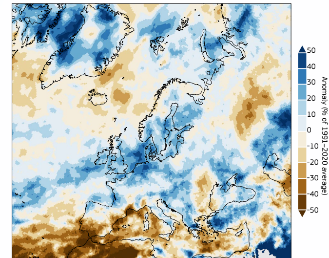
Annual precipitation anomalies (%) in 2023
