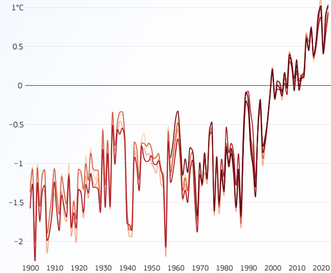
Anomalies in annual surface air temperature (°C) for European land (WMO RA VI Europe domain)
