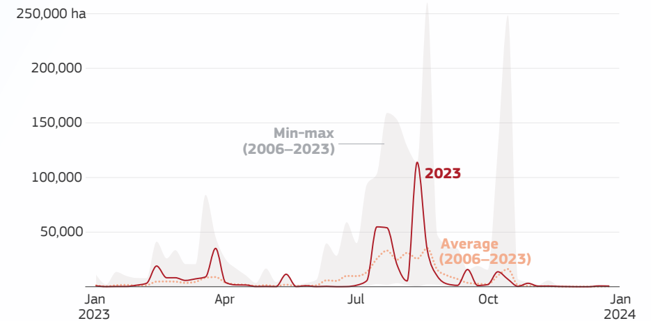
Weekly wildfire burnt areas (ha) in EU countries in 2023
