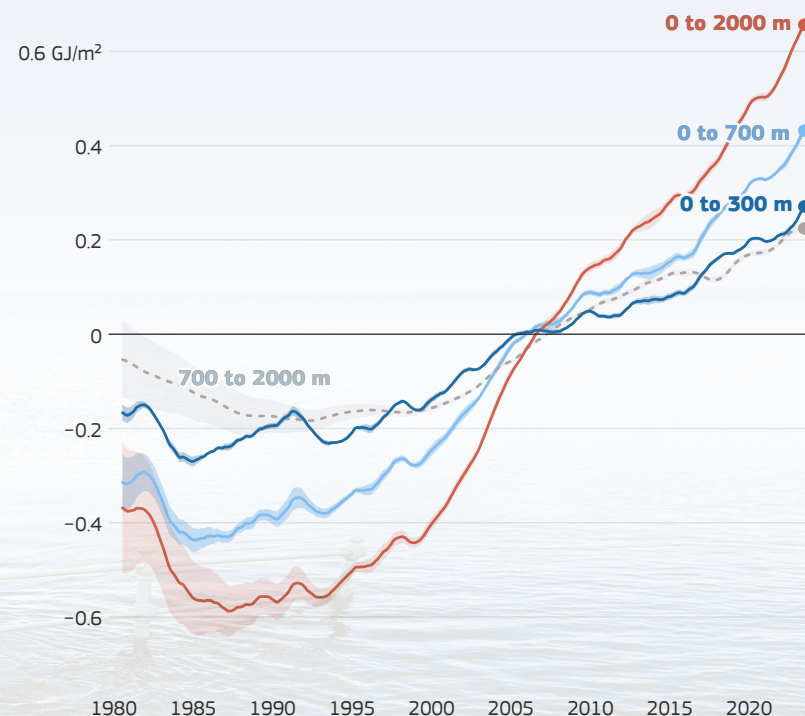
Anomalies (GJ/m²) in the heat content of the global ocean
