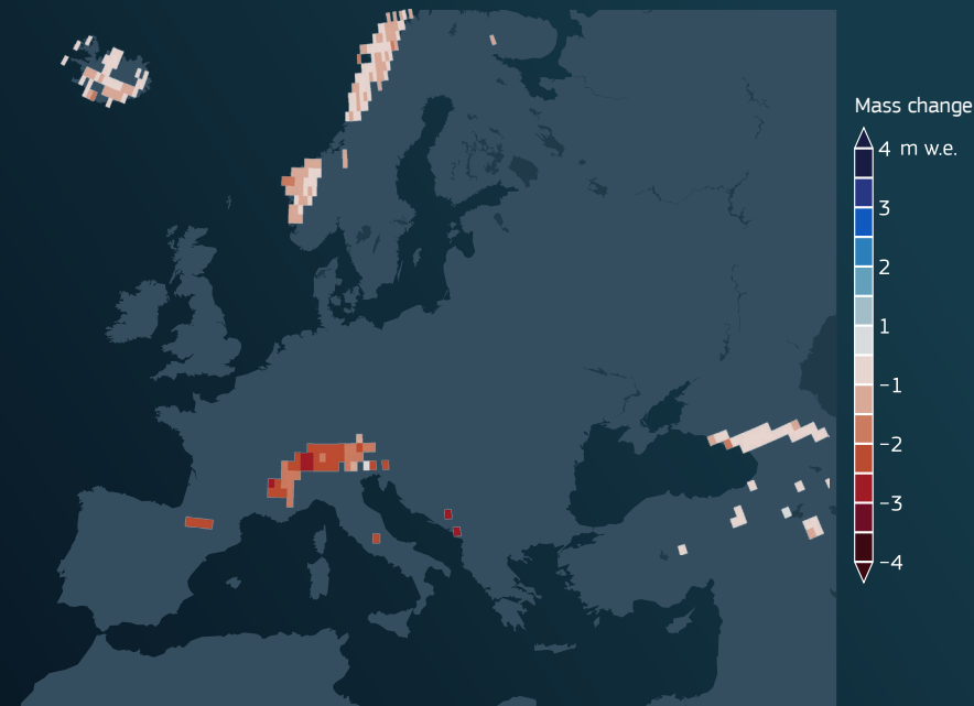
Mass change of glaciers across Europe in 2023
