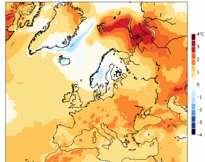
Average surface air temperature anomalies (°C) in 2023
