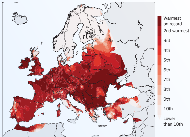
Ranking of annual average surface air temperatures in 2023
