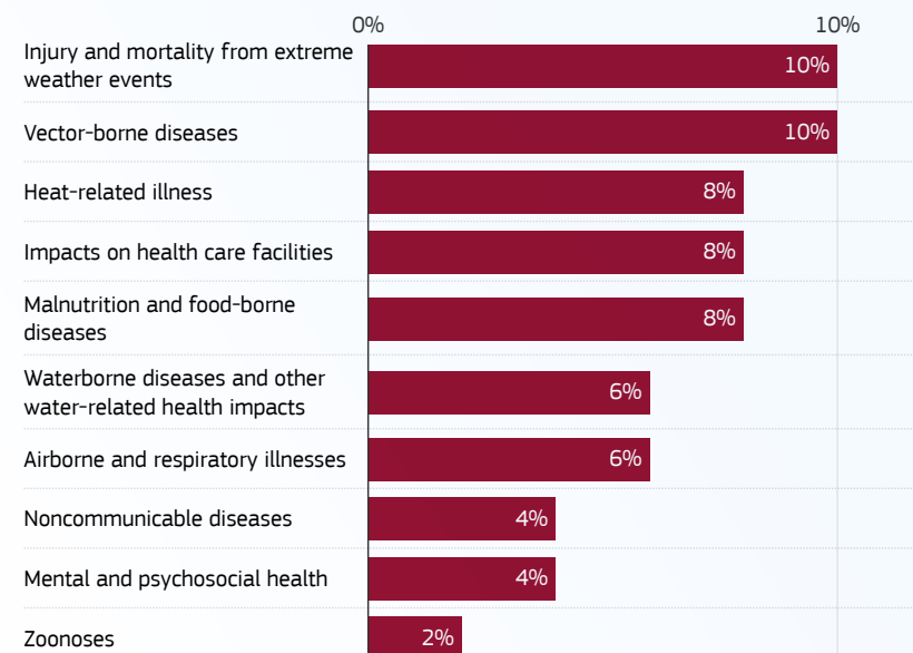
Percentage of European Member countries that refer to climate-sensitive health risks or outcomes in their Nationally Determined Contributions (NDCs) under the Paris Agreement
