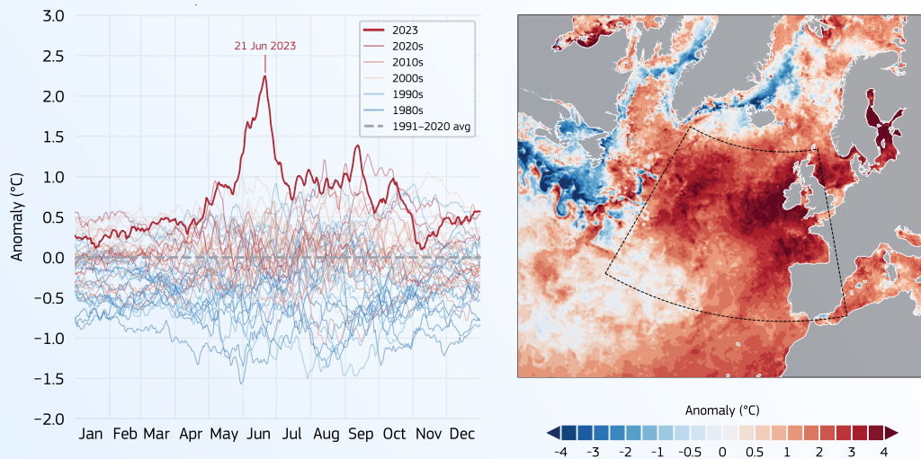
Daily sea surface temperature anomalies (°C) in the northeastern Atlantic Ocean from 1980 to 2023 (Left) · Daily sea surface temperature anomalies (°C) on 21 June 2023 (Right)
