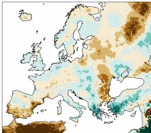
Anomalies (%) in soil moisture in 2023
