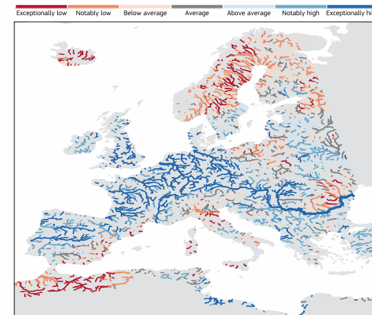
Anomalies in monthly average river flow in December 2023
