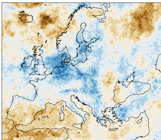
Anomalies in the number of wet days in 2023
