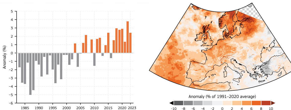
Anomalies (%) in annual solar radiation for European land (Left) - Anomalies (%) in solar radiation for 2023 (Right)
