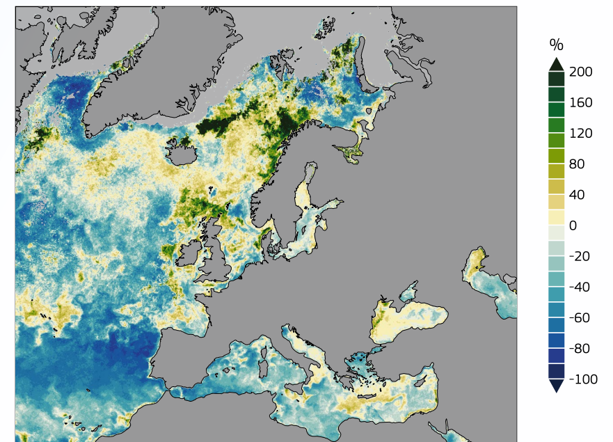
Anomalies in chlorophyll a concentration (%) in April 2023 Data source: C3S Ocean Colour v6.0 • Credit: C3S/ECMWF/Brockmann Consult
