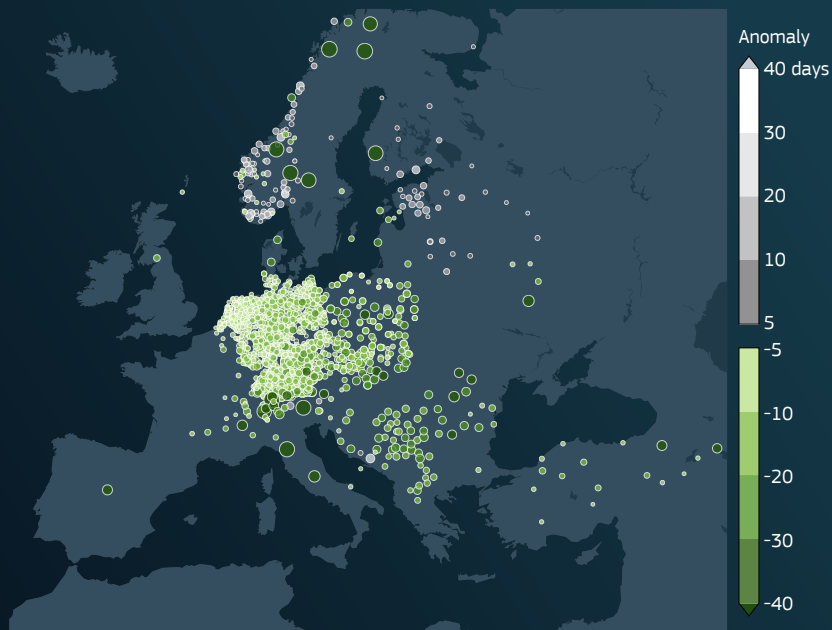
Anomalies in the number of snow days during winter (December 2022 to February 2023)
