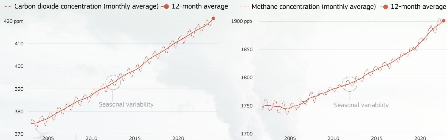
Global atmospheric concentrations of carbon dioxide (CO 2 ) and methane (CH 4 )
