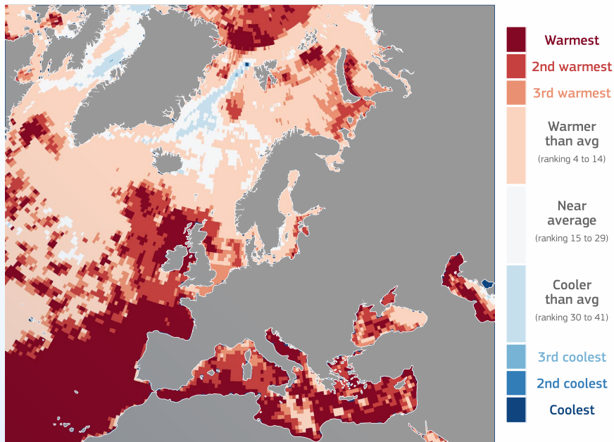
Ranking of the annual average sea surface temperatures in 2023 Data source: ESA SST CCI Analysis v3.0 • Credit: ESACCI/EOCIS/UKMCAS and C3S/ECMWF
